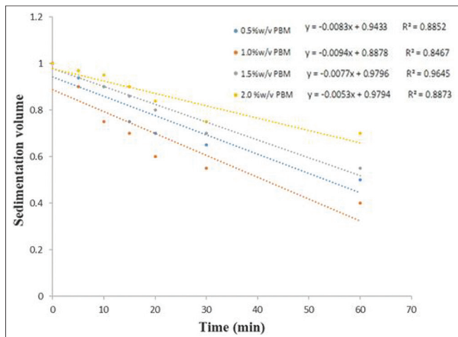
Figure 1: Sedimentation profiles of different Parkia biglobosa mucilage-based suspensions.
