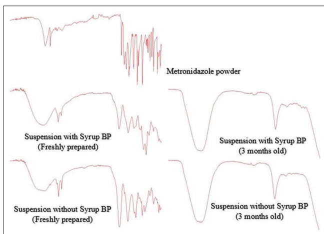
Figure 3: Fourier-transform infrared spectroscopy of pure metronidazole and the optimized formulation (with and without Syrup BP) when freshly prepared and after 3 months of storage at ambient temperature.
