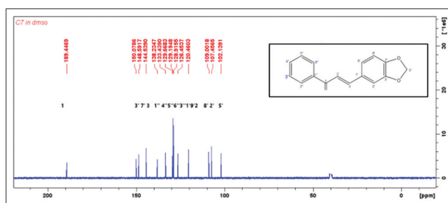
Figure S2: 13 C NMR of compound C2
