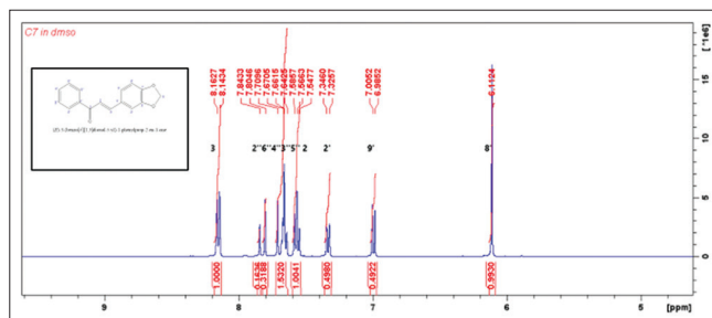
Figure S1: 1 H NMR of Compound C2
